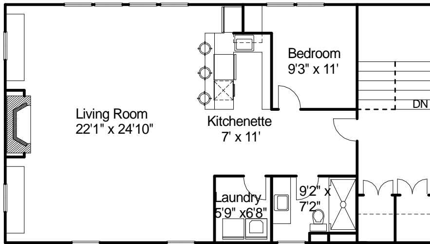
Carriage House Second Floor
