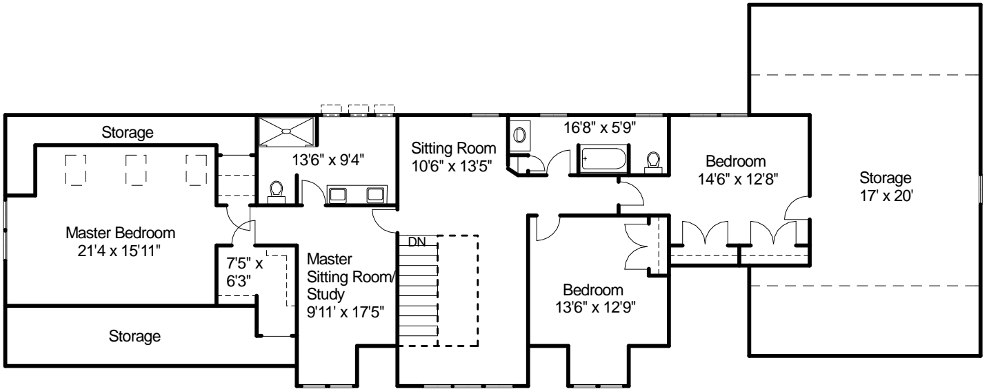
Second Floor
