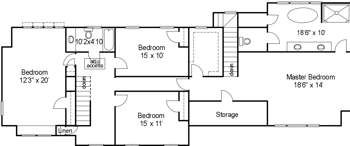
Second Floor
