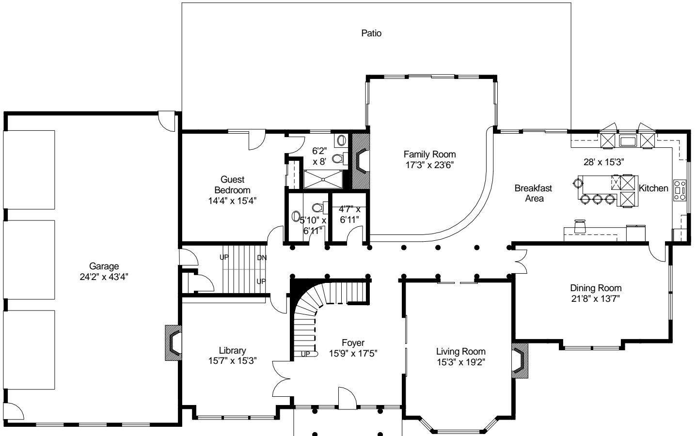
First Floor
