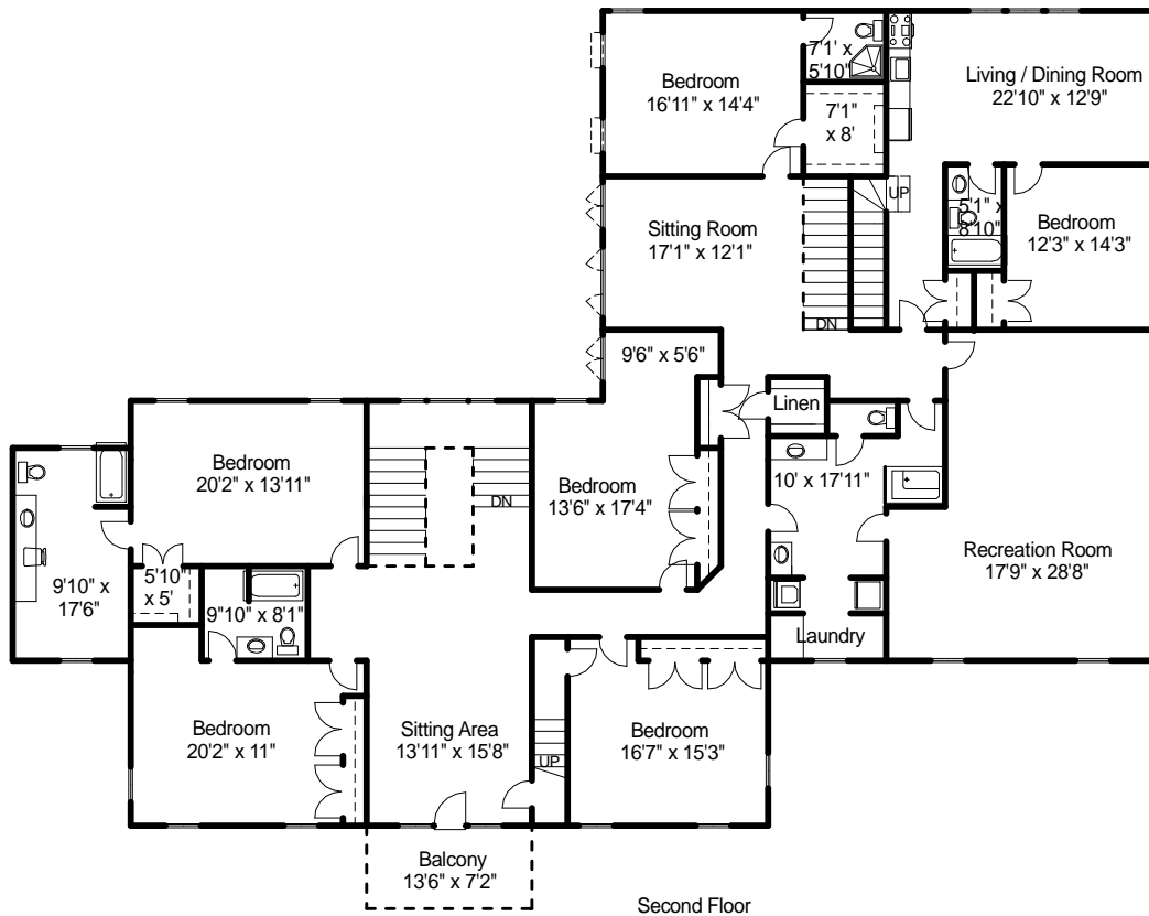
Second Floor
