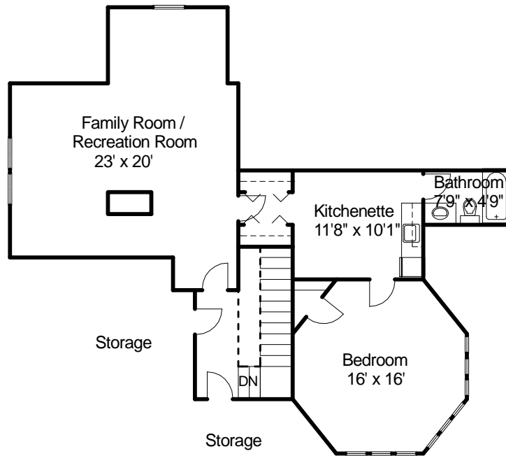
Third Floor
