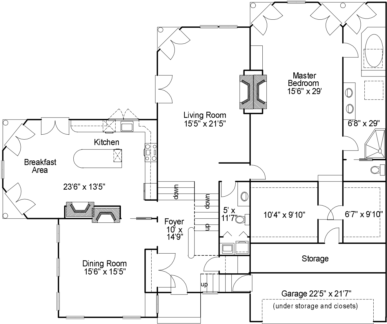
First Floor
